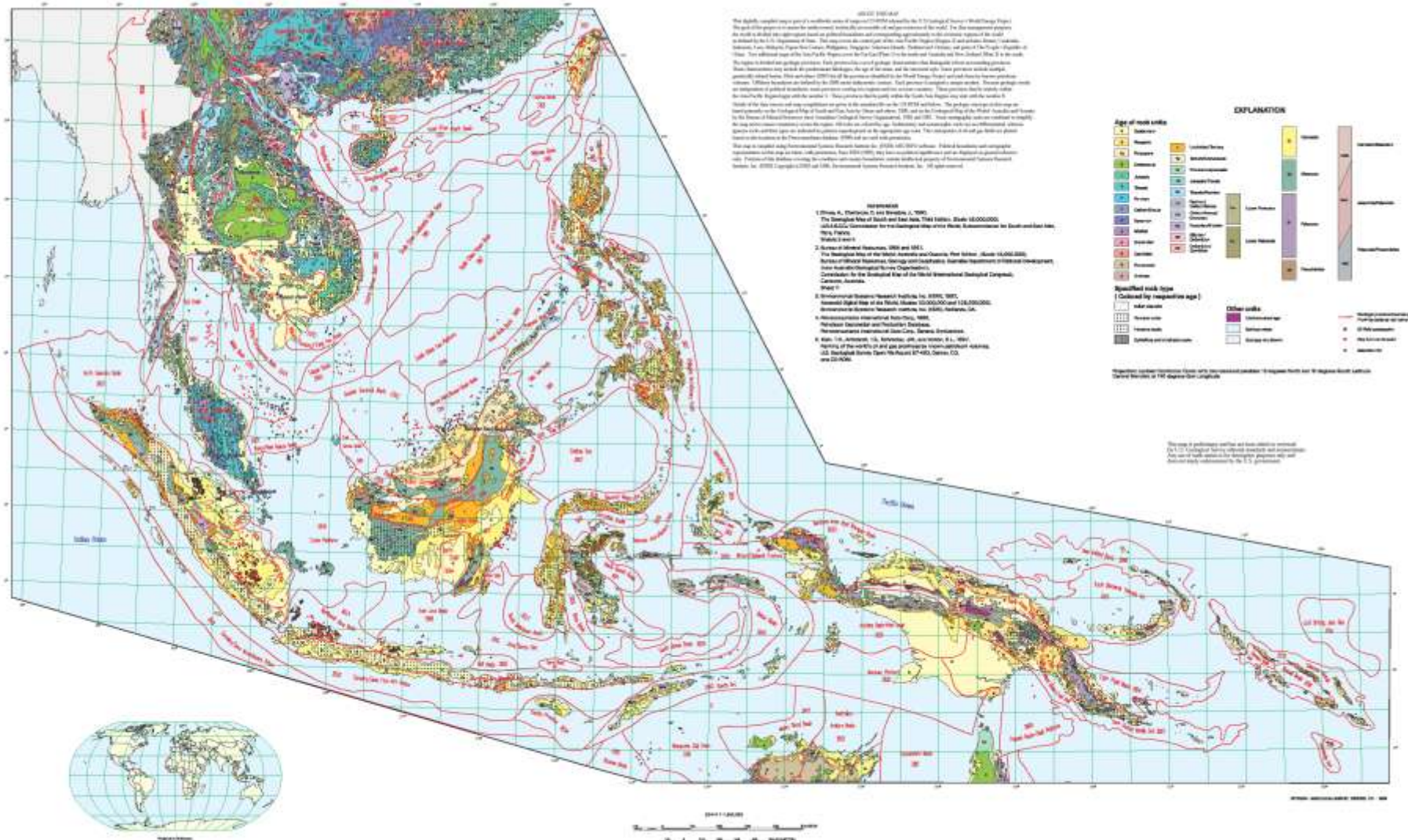
MAPS SHOWING GEOLOGY, OIL AND GAS FIELDS AND GEOLOGIC PROVINCES OF THE ASIA PACIFIC REGION
